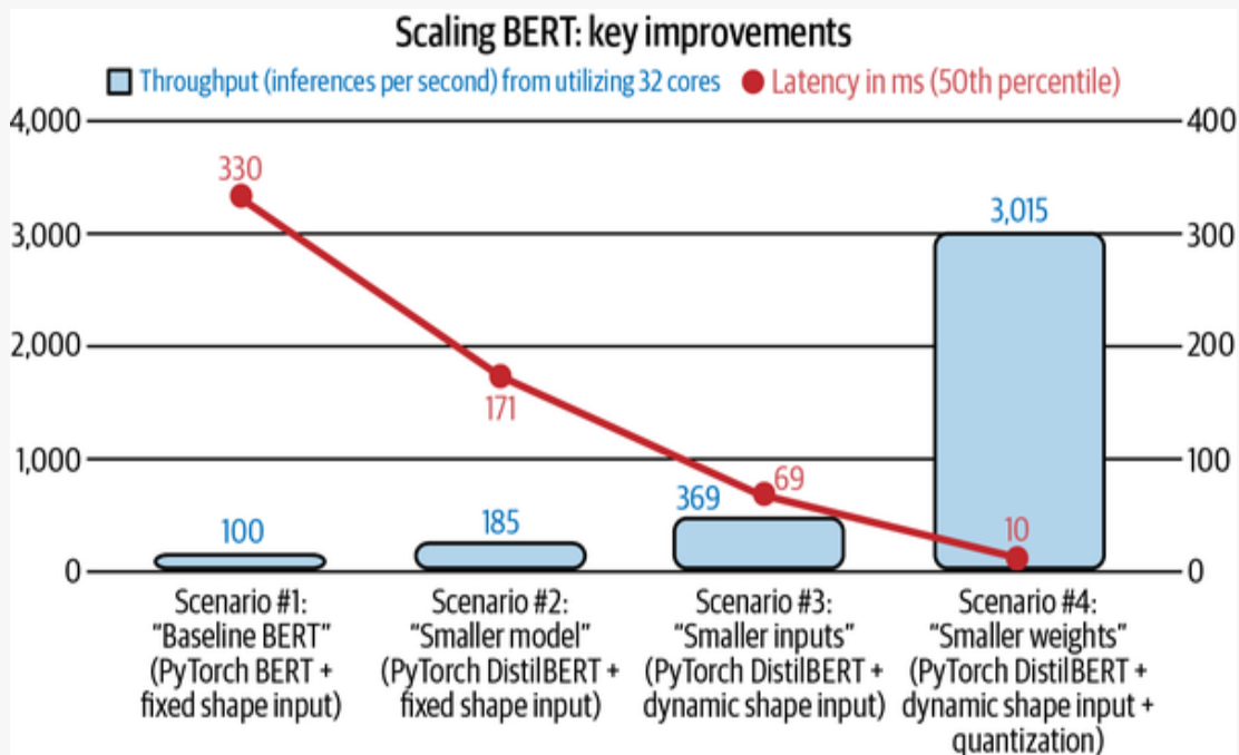
Figure 7-10. Latency improvement by various model compression methods. Source: Adapted from an image by Le and Kaehler
