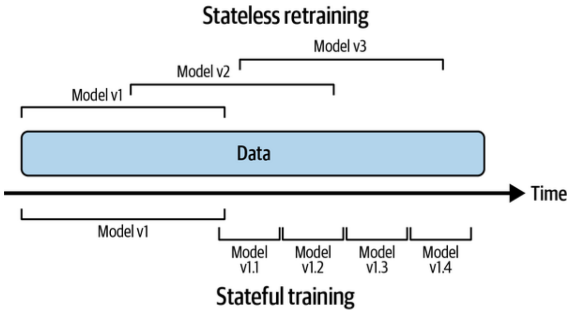
Figure 9-2. Stateless retraining versus stateful training
