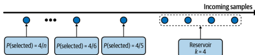
Figure 4-2. A visualization of how reservoir sampling works
