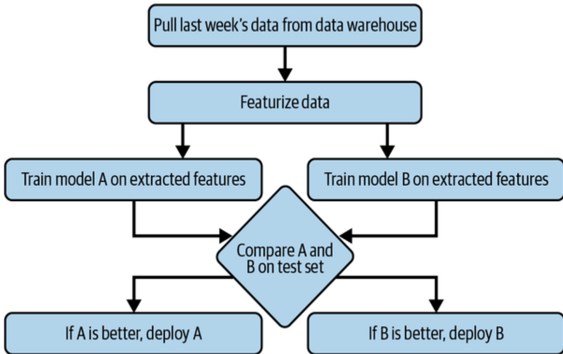
Figure 10-7. A graph that shows the order of execution of a simple ML workflow, which is essentially a DAG (directed acyclic graph)
