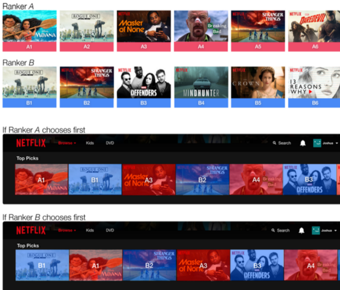
Figure 9-7. Interleaving video recommendations from two ranking algorithms using team draft. Source: Parks et al. 32
