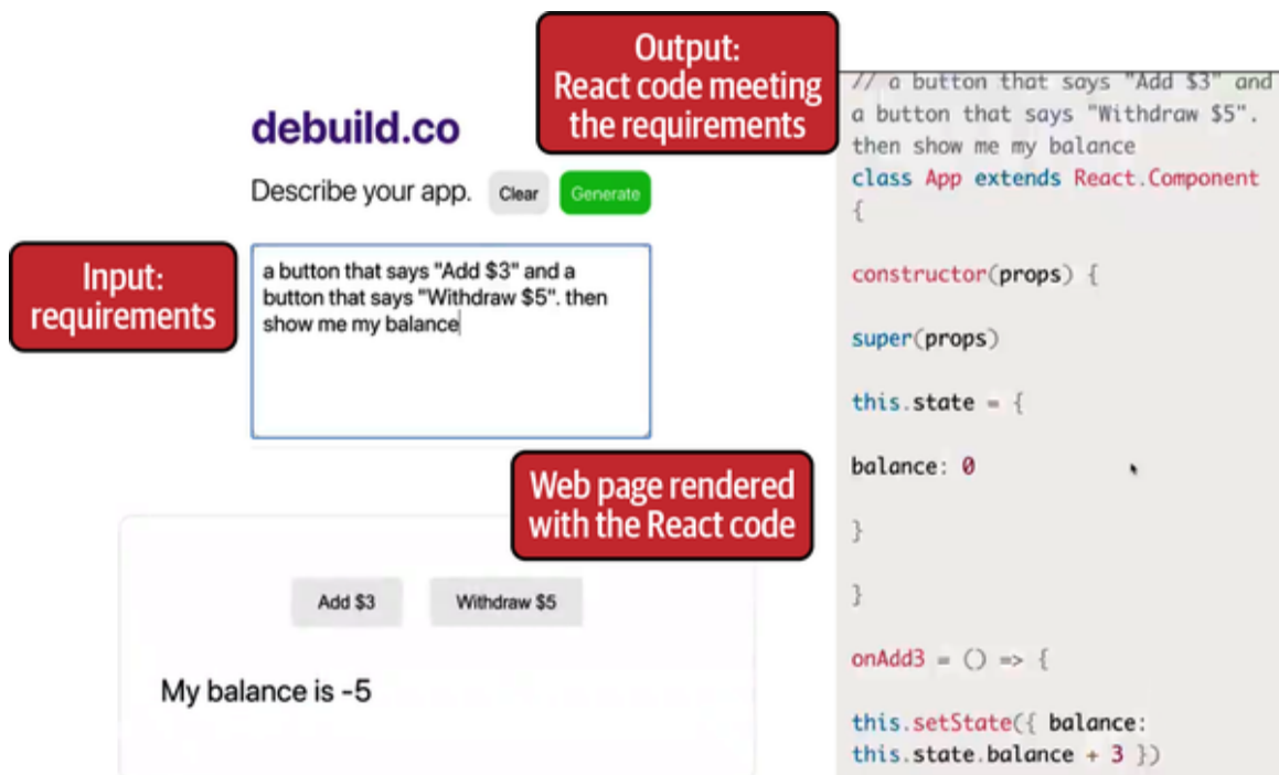
Figure 11-1. GPT-3 can help you write code for your website. Source: Adapted from screenshots of a video by Sharif Shameem
