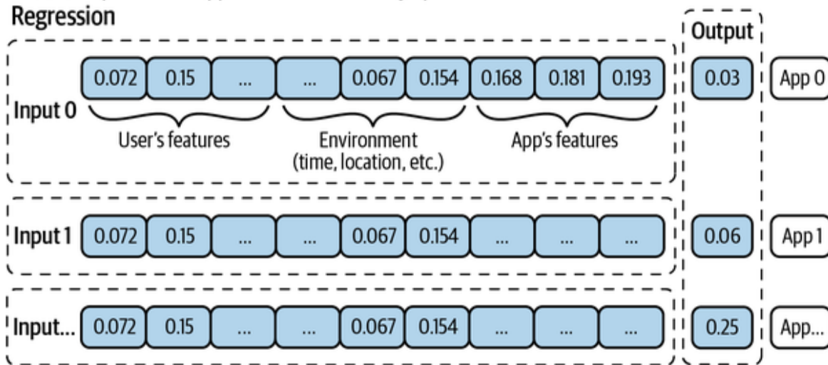
Figure 2-6. Given the problem of predicting the app a user will most likely open next, you can frame it as a regression problem. The input is the user's features, environment's features, and an app's features. The output is a single value between 0 and 1 denoting how likely the user will be to open the app given the context.
