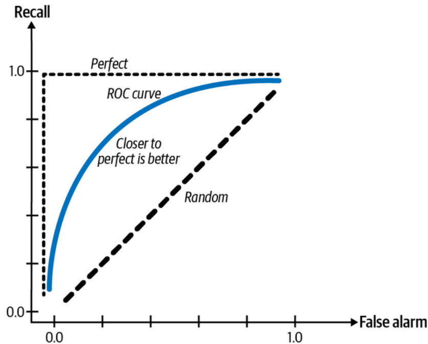
Figure 4-9. ROC curve
