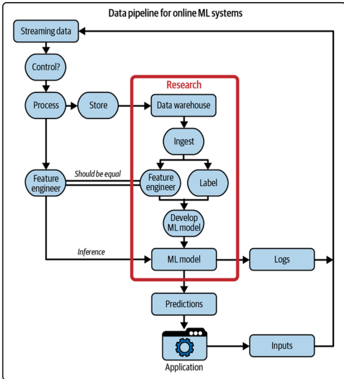
Figure 7-8. A data pipeline for ML systems that do online prediction
