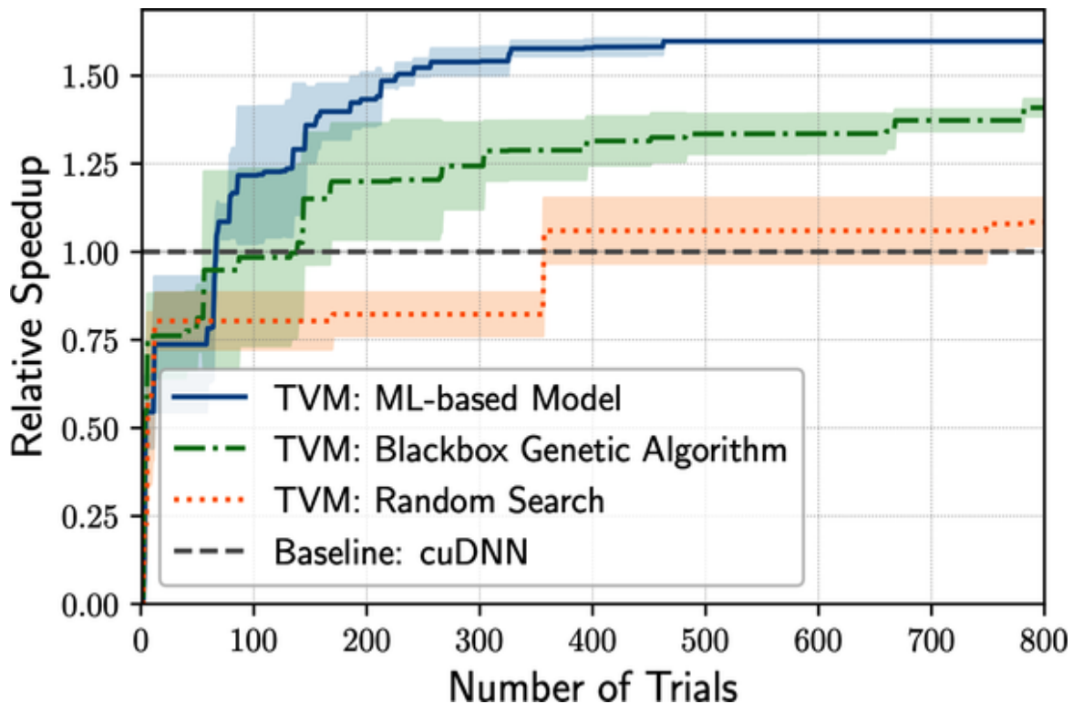
Figure 7-15. Speedup achieved by autoTVM over cuDNN for ResNet-50 on NVIDIA TITAN X. It takes ~70 trials for autoTVM to outperform cuDNN. Source: Chen et al. 50
