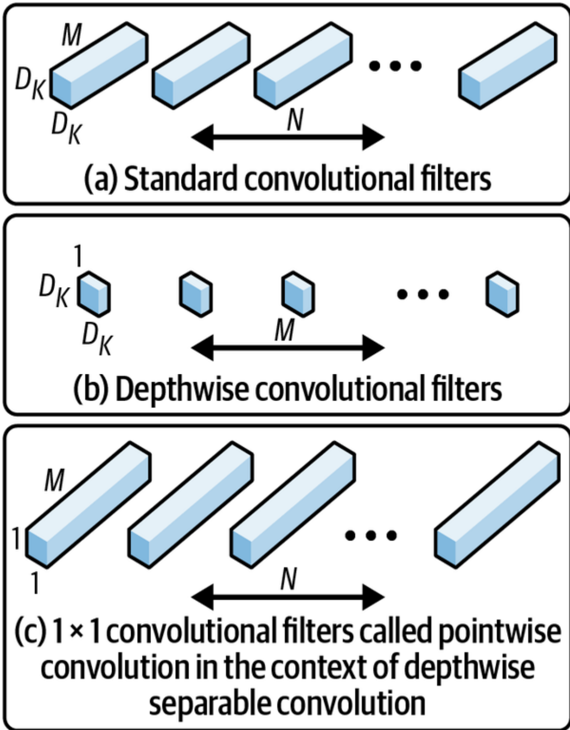
Figure 7-9. Compact convolutional filters in MobileNets. The standard convolutional filters in (a) are replaced by depthwise convolution in (b) and pointwise convolution in (c) to build a depthwise separable filter. Source: Adapted from an image by Howard et al.
